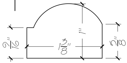
BULLNOSE DETAIL SCALE: FULL
